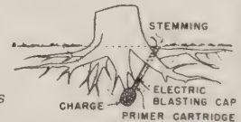
FIG. 218—In Loading a Small Lateral Rooted Stump the Charge Should Be Kept Well Down
